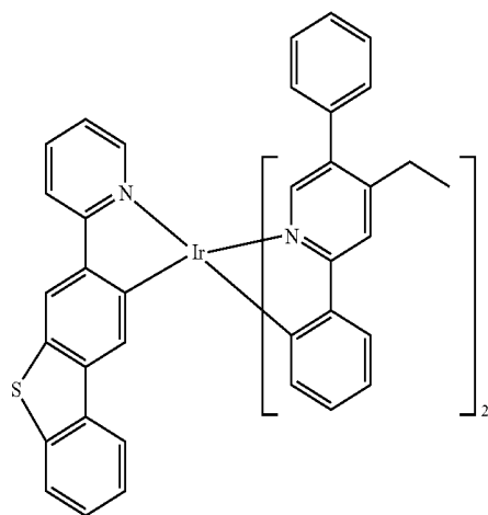
Compound 65
