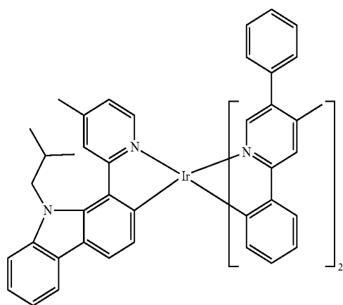
Compound 88
