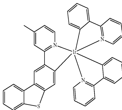
Compound 21
