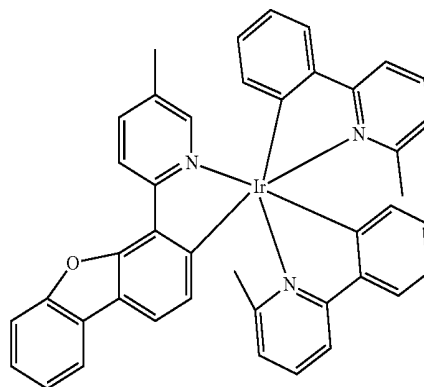
Compound 58
