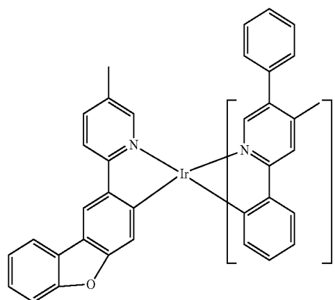
Compound 45
