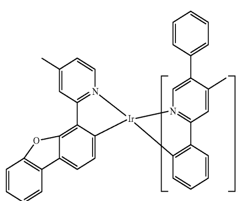
Compound 40
