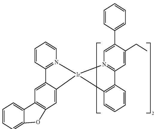
Compound 48
