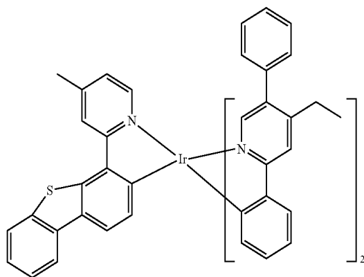
Compound 73
