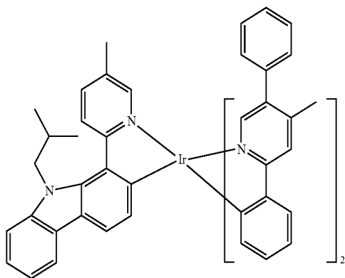
Compound 91
