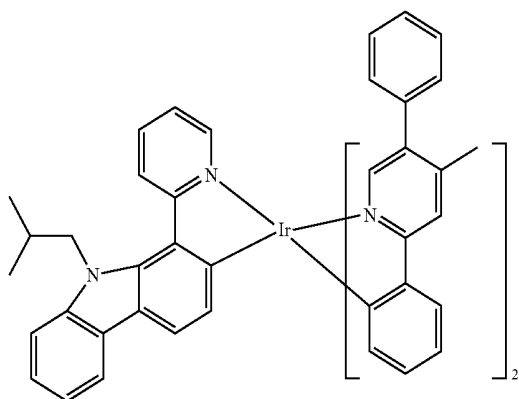
Compound 85
