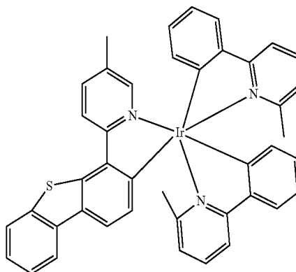
Compound 82
