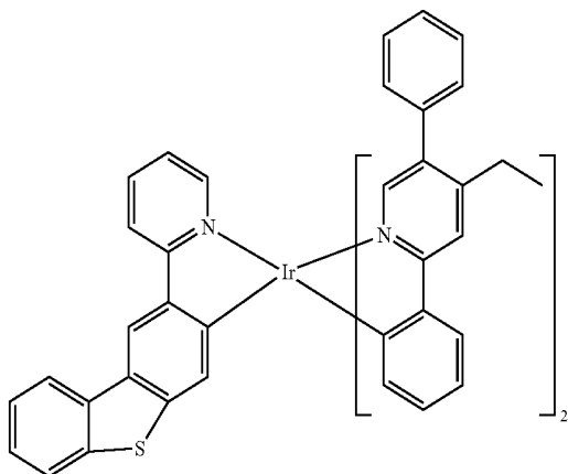
Compound 72
