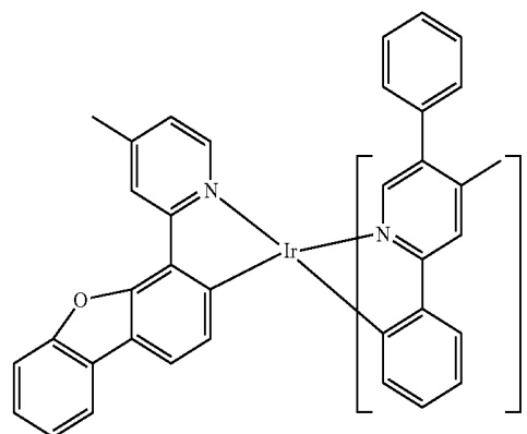
Compound 40
