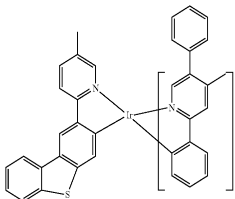
Compound 69
