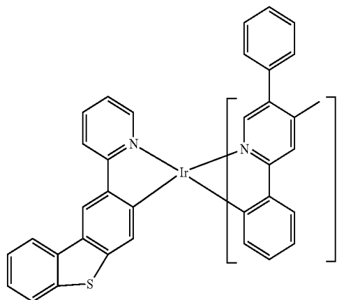
Compound 63
