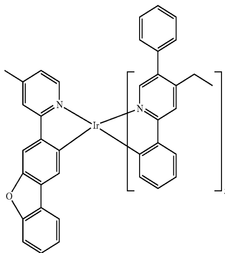
Compound 50
