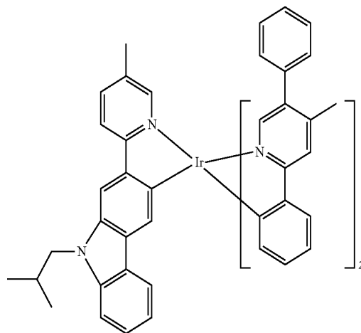
Compound 92
