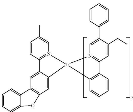
Compound 54
