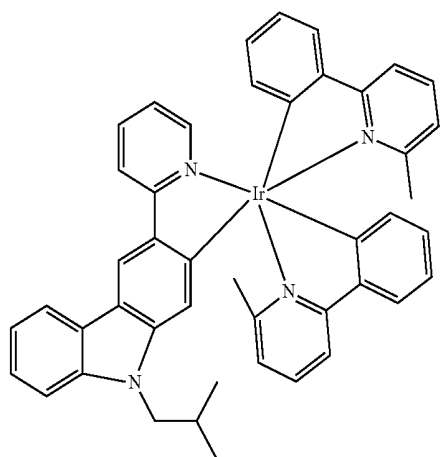
Compound 30
