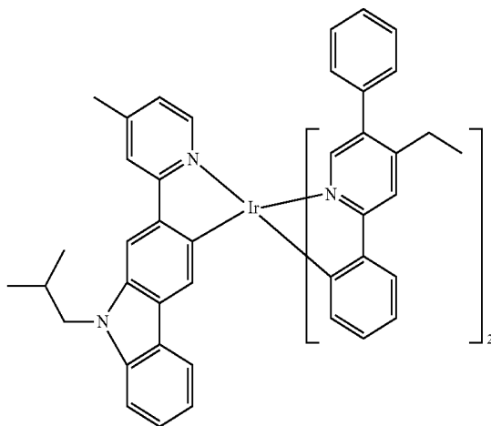
Compound 98
