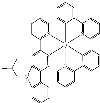
Compound 104
