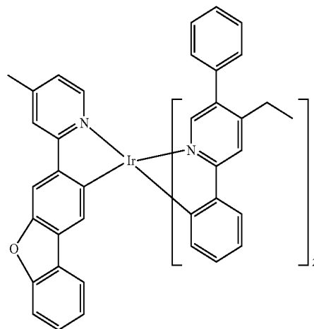
Compound 50
