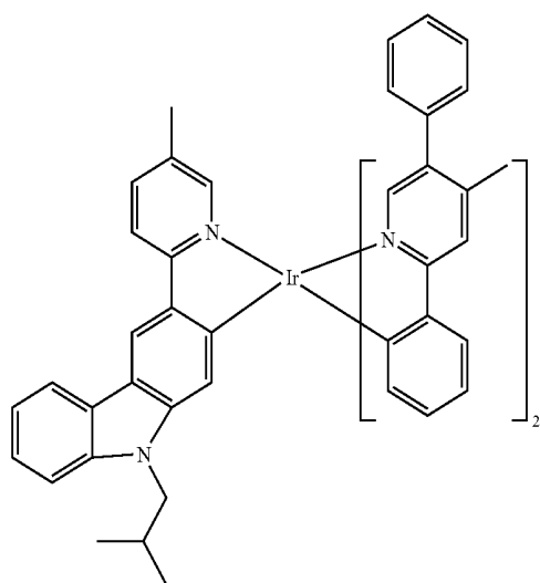
Compound 93
