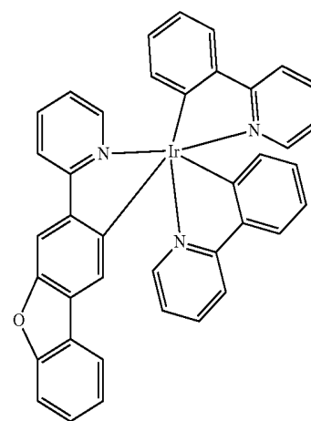
Compound 2
