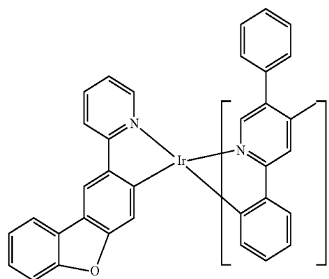
Compound 39
