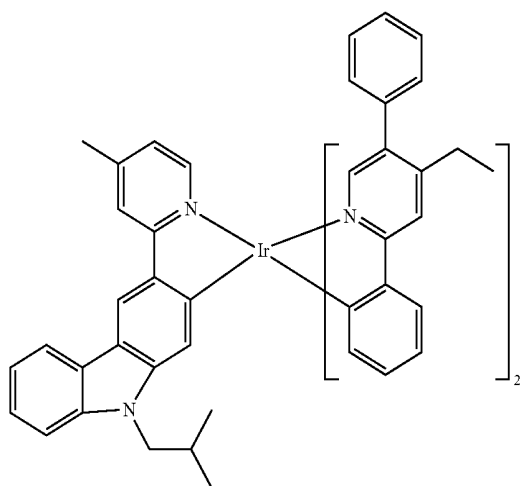
Compound 99
