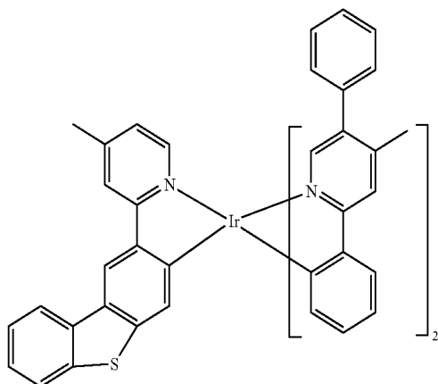
Compound 66
