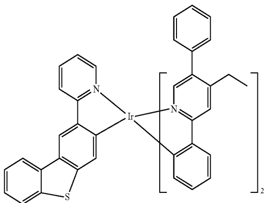
Compound 72
