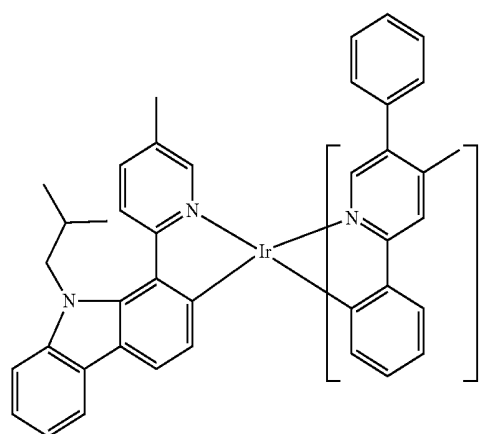
Compound 91
