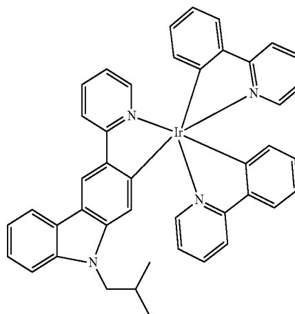
Compound 27
