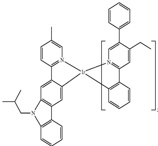
Compound 101
