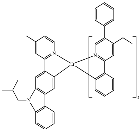
Compound 98
