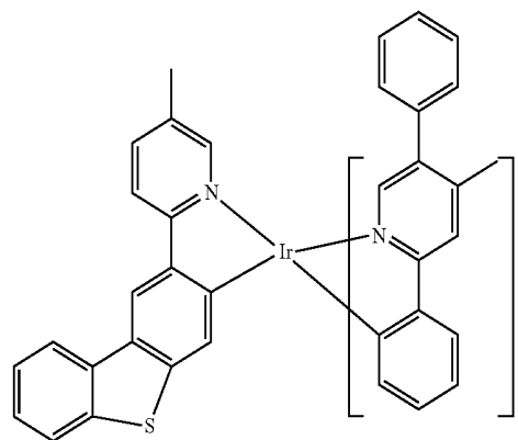
Compound 63
