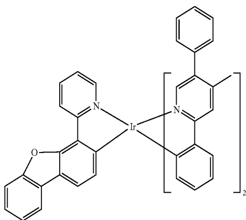
Compound 37
