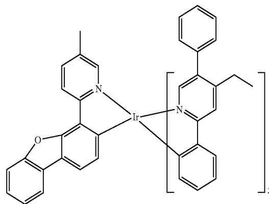
Compound 52
