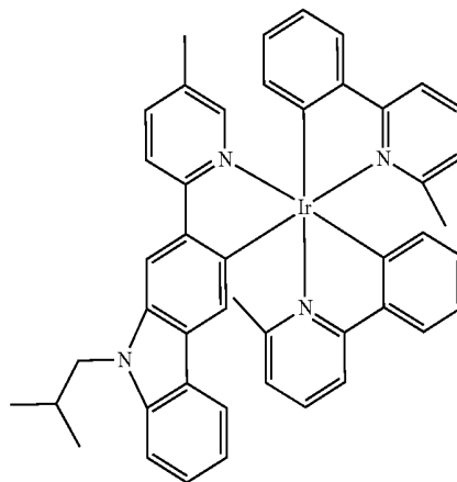
Compound 108
