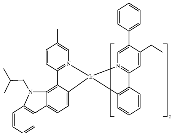
Compound 100
